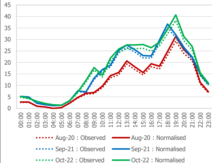
Skinner Street : Average Daily Motorcycle Flows
