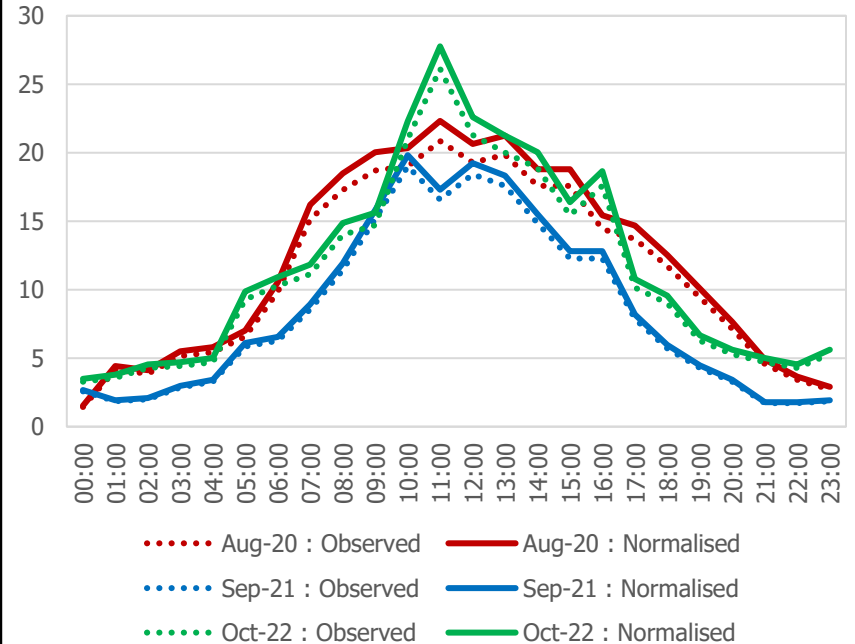
St John Street (south of Rosebery Ave) : Average Daily LGV Flows
