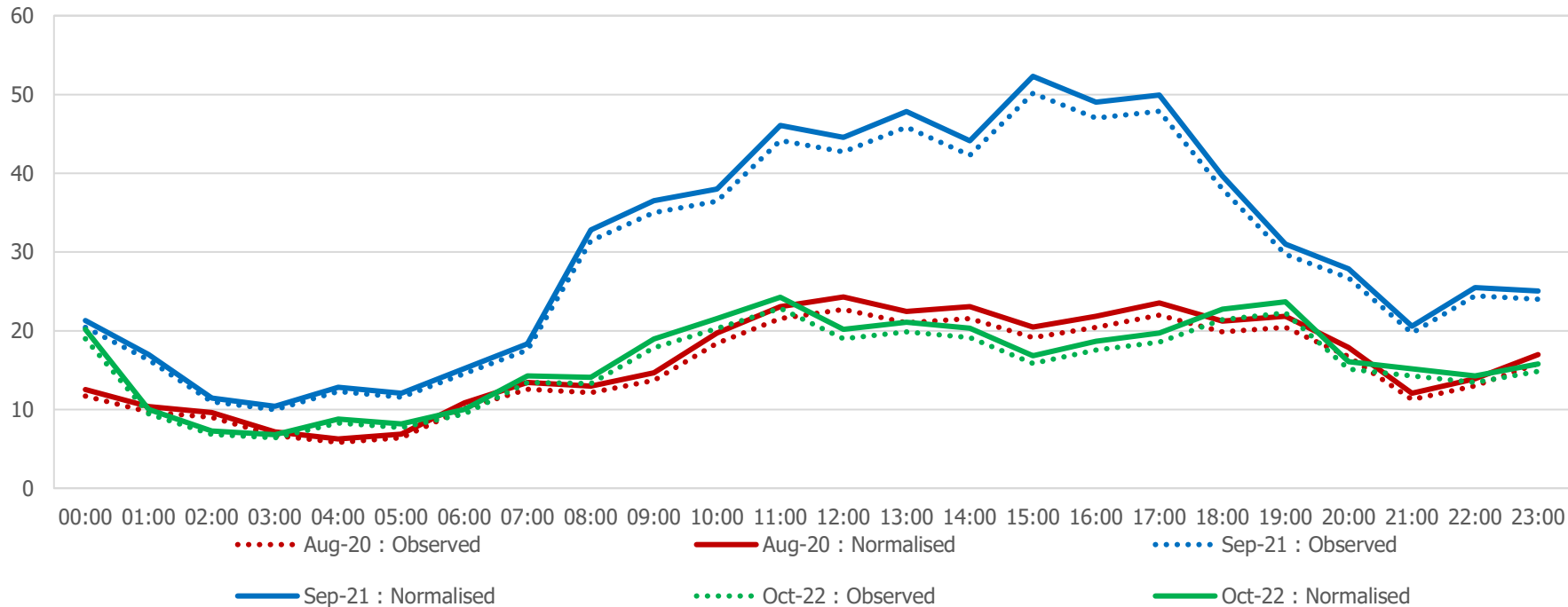
Cowcross Street : Average Daily Car Flows
