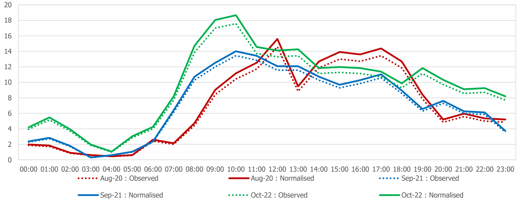
Sekforde Street : Average Daily Car Flows
