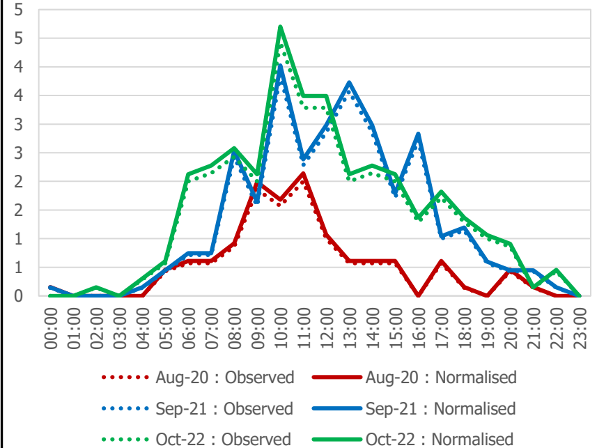
Woodbridge Street : Average Daily LGV Flows
