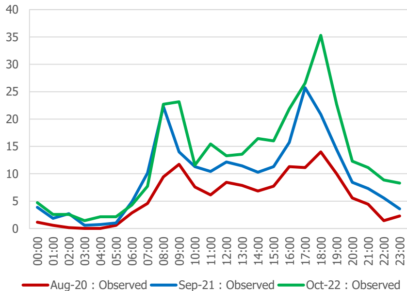
Clerkenwell Green (west site, eastbound) : Average Daily Cycle Flows
