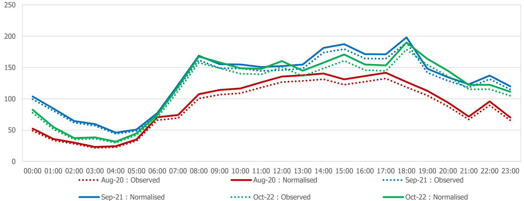
St John Street (south of Rosebery Ave) : Average Daily Car Flows
