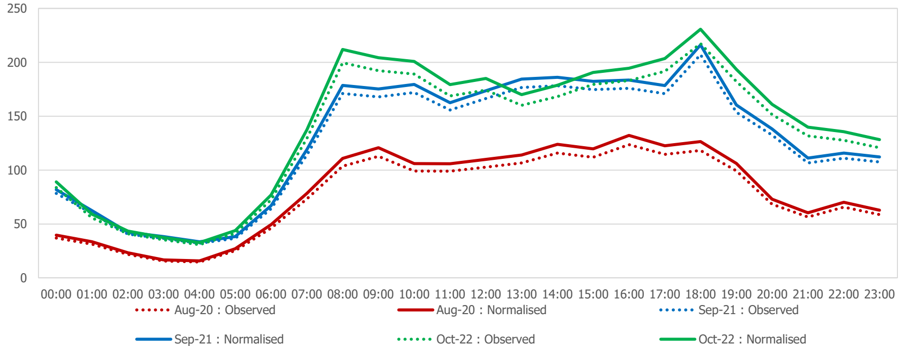
St John Street (near Great Sutton St) : Average Daily Car Flows
