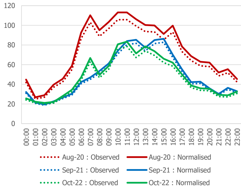
Rosebery Avenue : Average Daily LGV Flows
