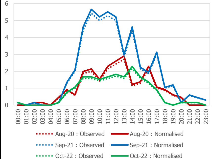
Sekforde Street : Average Daily LGV Flows
