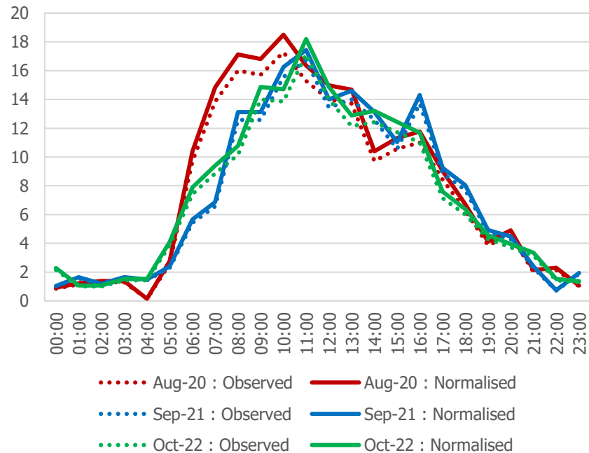
Spencer Street : Average Daily LGV Flows
