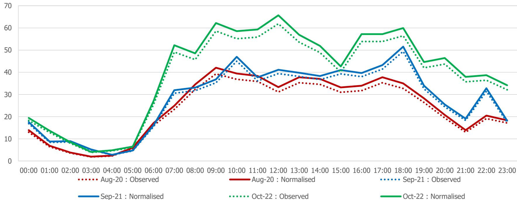
Clerkenwell Green (west site, eastbound) : Average Daily Car Flows
