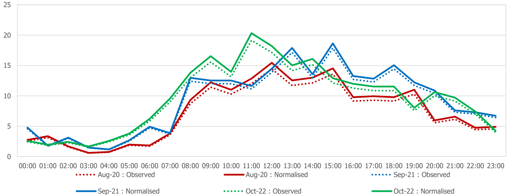
Clerkenwell Close : Average Daily Car Flows
