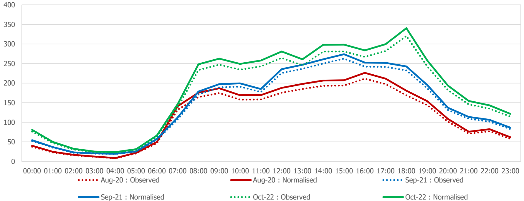
Skinner Street : Average Daily Car Flows
