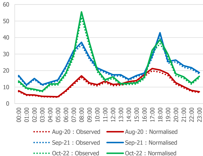
Rosebery Avenue : Average Daily HGV Flows
