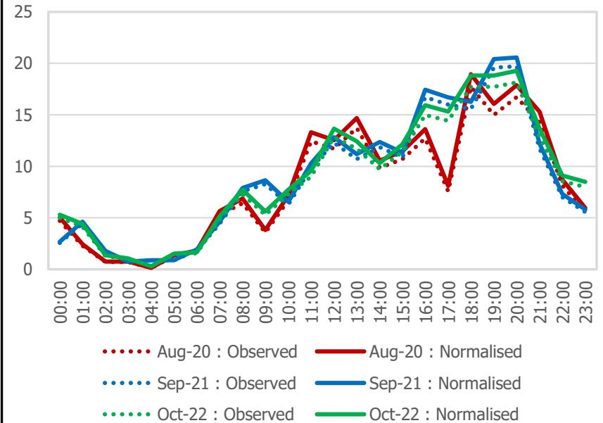
St John Street (south of Rosebery Ave) : Average Daily Motorcycle Flows
