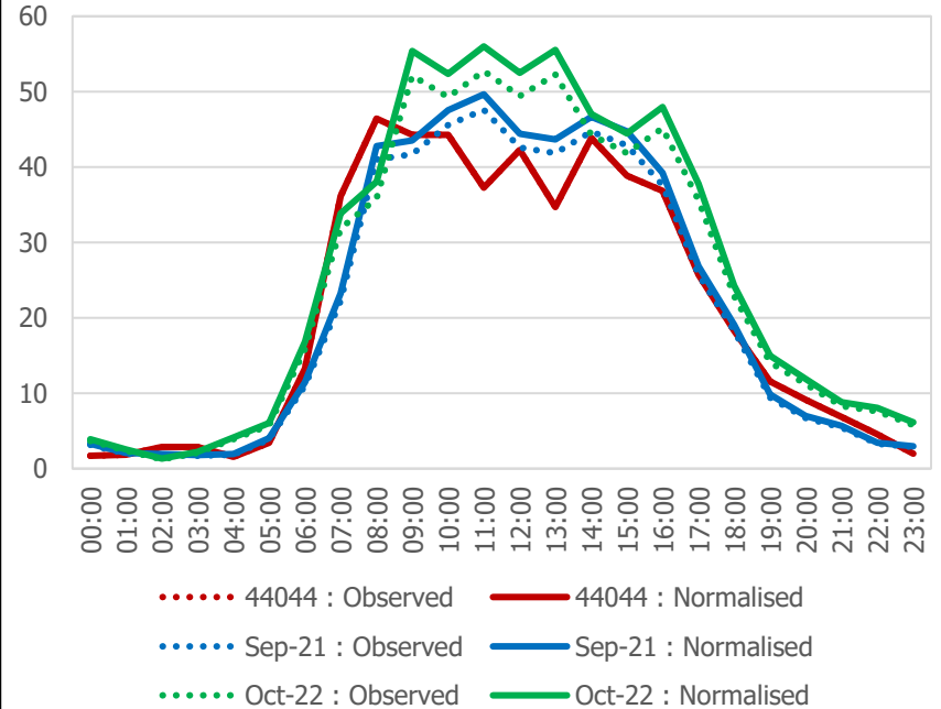
Percival Street : Average Daily LGV Flows
