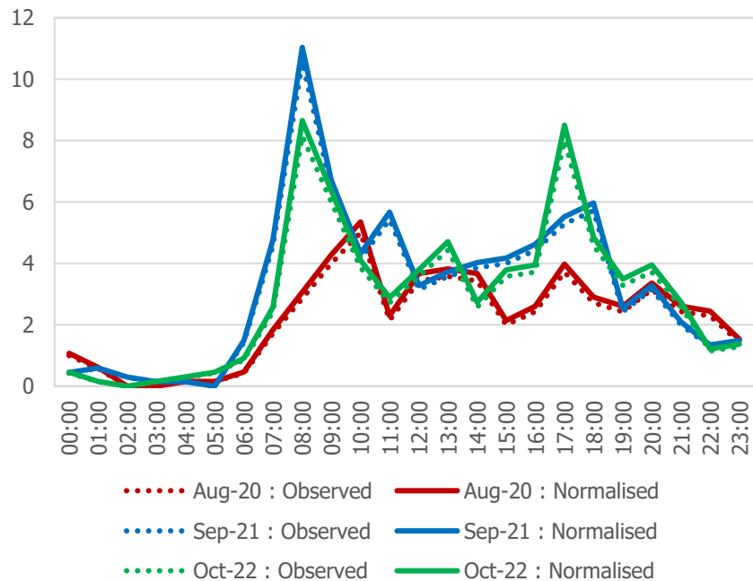
Skinner Street : Average Daily HGV Flows
