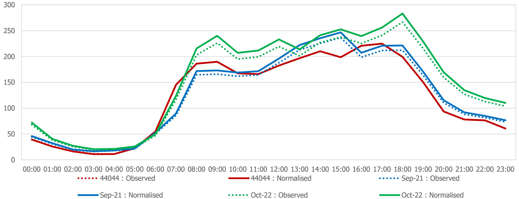
Percival Street : Average Daily Car Flows
