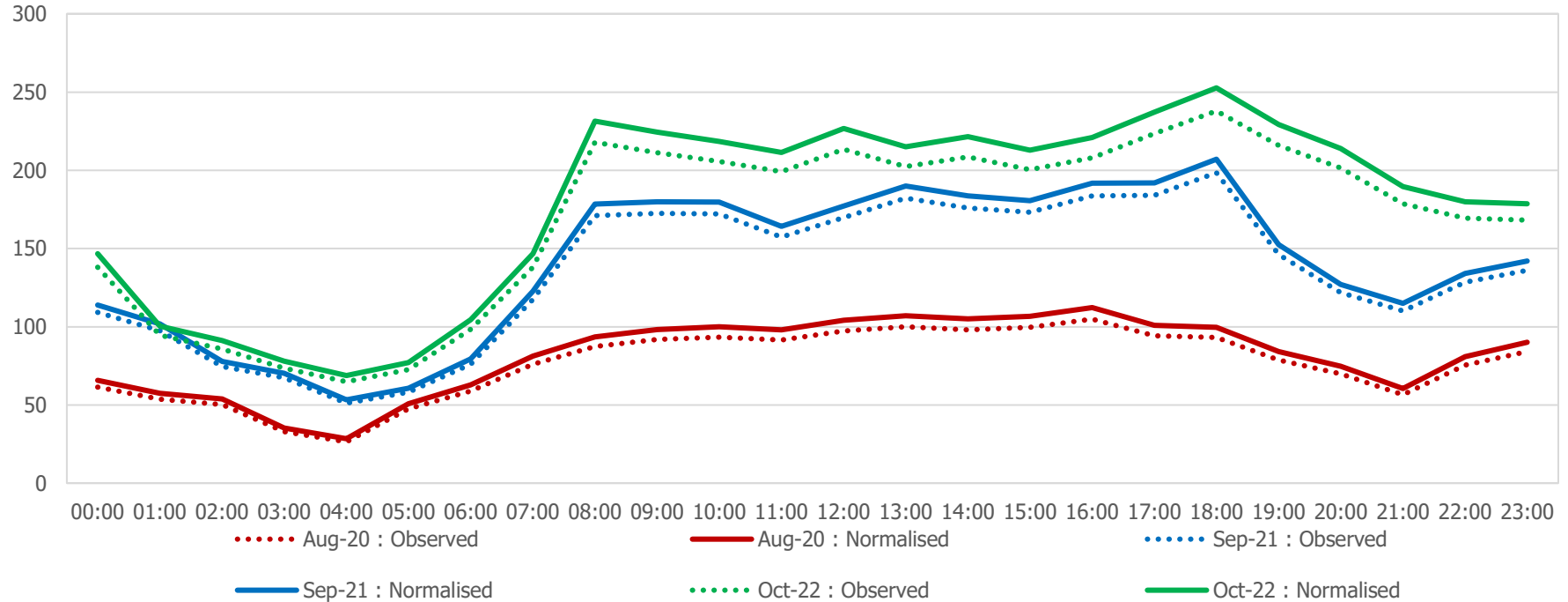
St John Street (near Passing Alley) : Average Daily Car Flows
