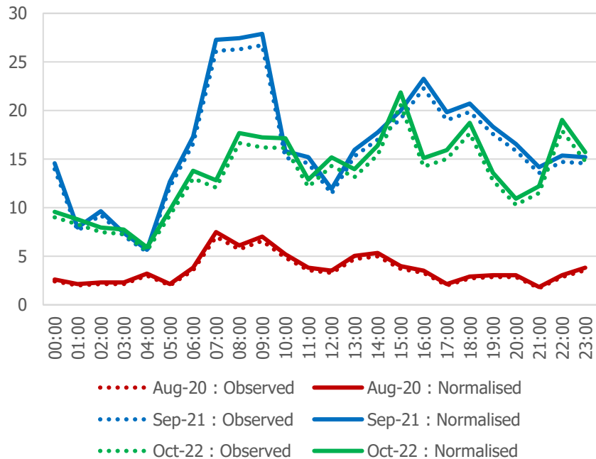
Farringdon Lane : Average Daily HGV Flows
