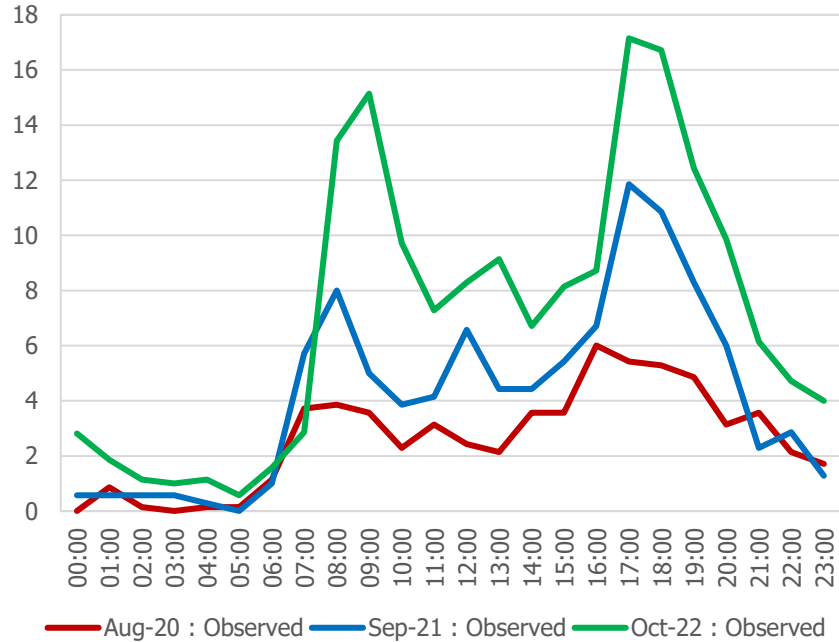
Sekforde Street : Average Daily Cycle Flows
