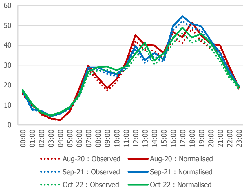
Rosebery Avenue : Average Daily Motorcycle Flows
