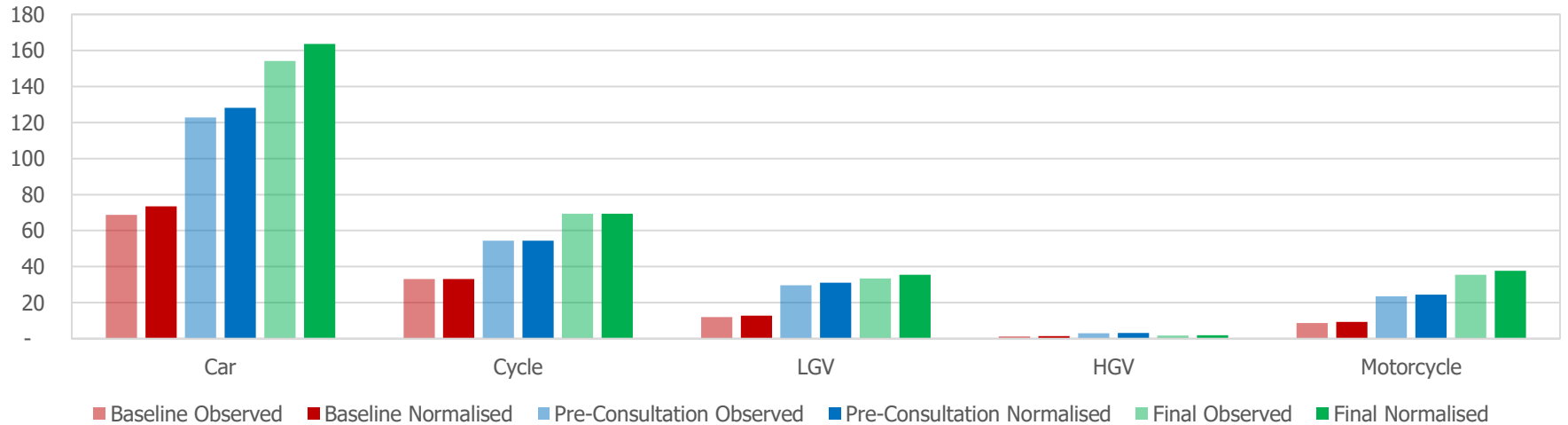
Woodbridge Street : Average Flows by Stage
