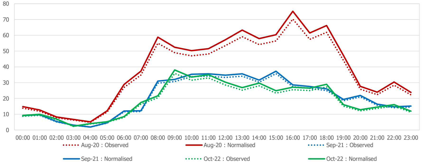
Bowling Green Lane : Average Daily Car Flows
